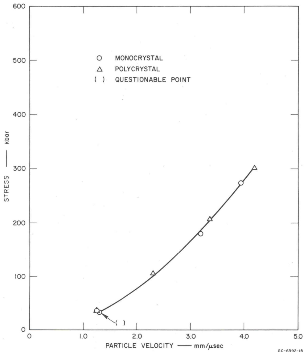
FIG. 18 HUGONIOT DATA FOR ICE ( \sigma - u )
